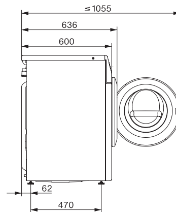
W1 drawing, slanted facia, straight facia, measures in mm
